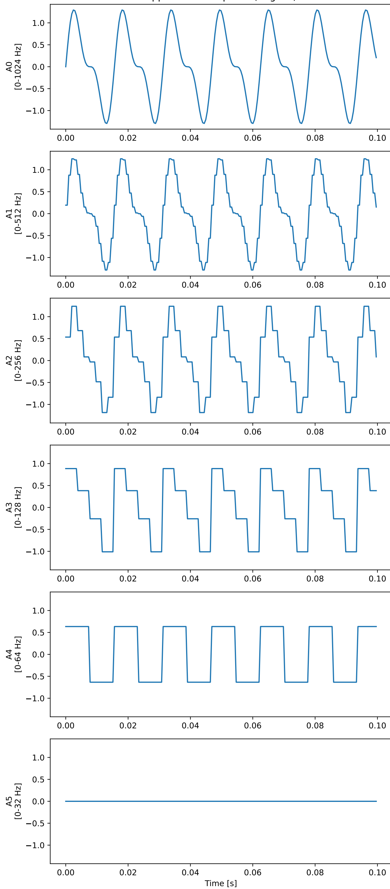
Approximation spaces (original)
