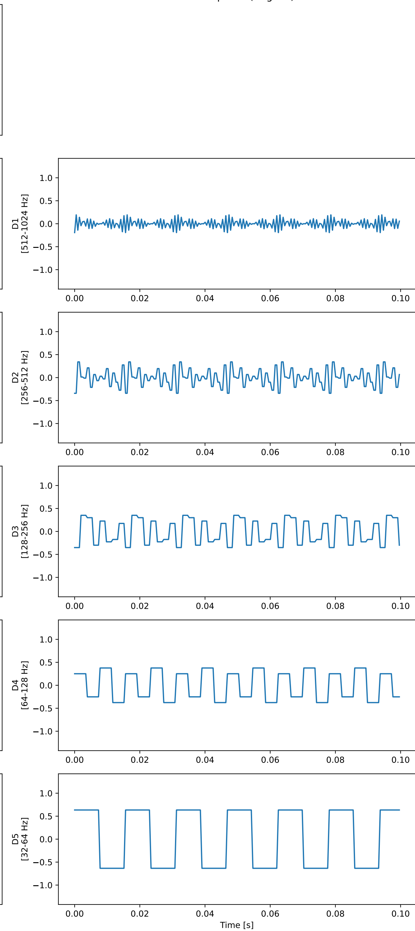
Detail spaces (original)
